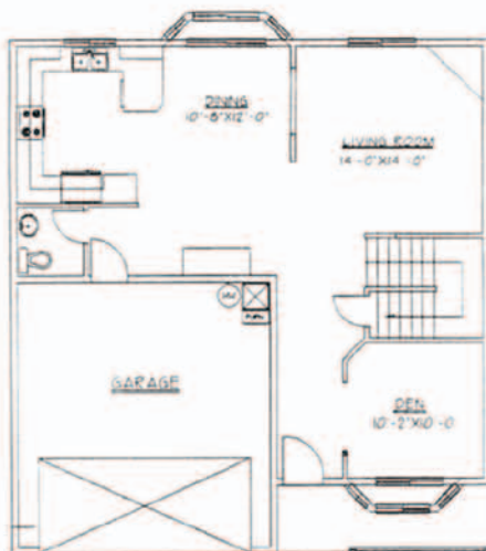
Main Level
