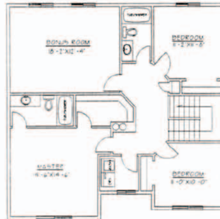
Upper Level
